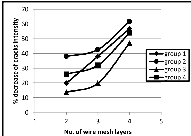
Fig. 15: Effect of number of wire mesh layers on cracks intensity
