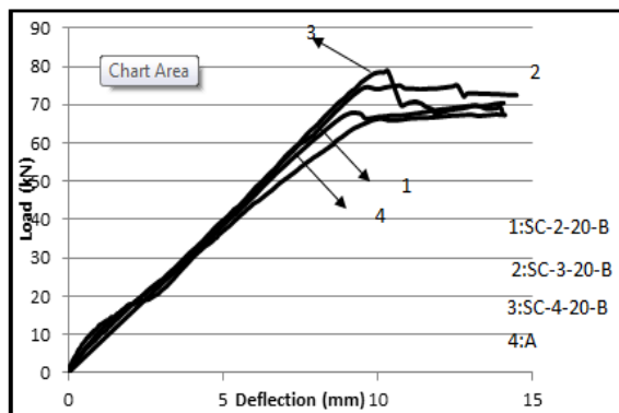
Fig. 9: Load-deflection curve of group1
