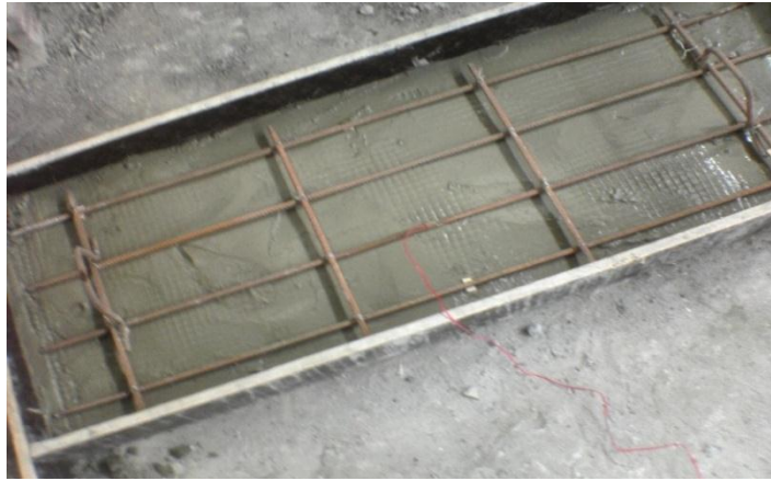
Fig 3: Placing the reinforcement
