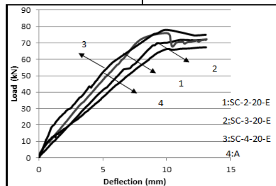
Fig. 10: Load-deflection curve of group2
