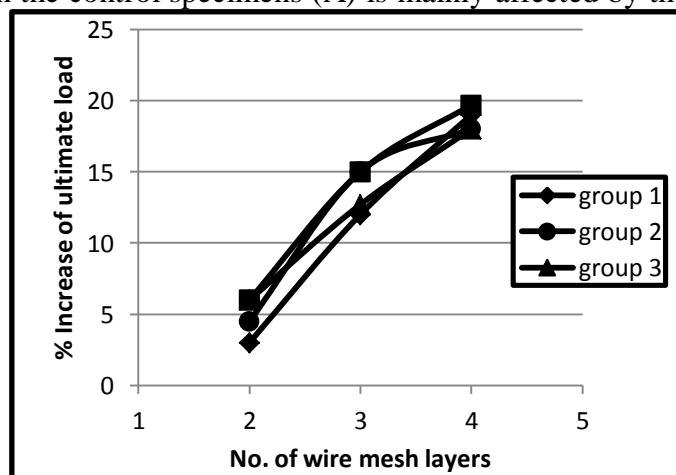
Fig. 13: Effect of number of wire mesh layers on the ultimate load
