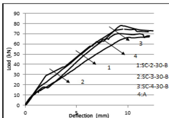
Fig. 11: Load-deflection curve of group3
