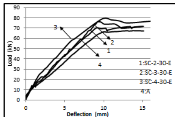
Fig. 12: Load-deflection curve of group4
