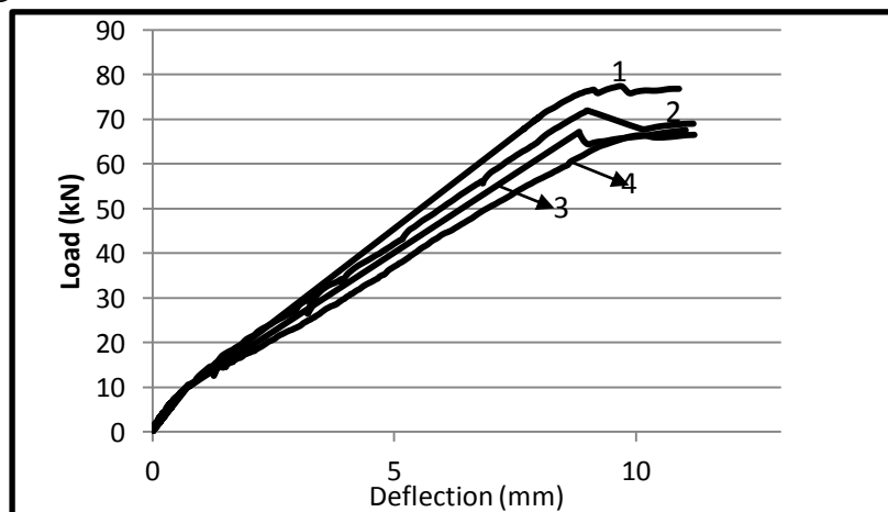
Fig. 8: Load-deflection curve of strengthened slabs
